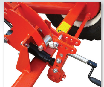
Hydraulically controlled braking system
