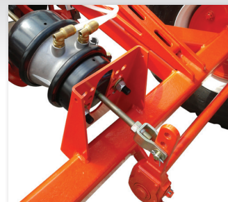
Pneumatically controlled braking system
